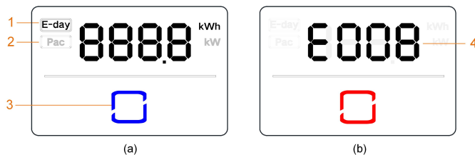
figure 2-4 Panneau LED
