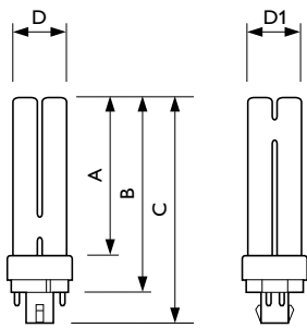
PL-C Xtra 26W/840/4P
