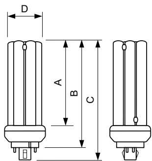
PL-T TOP 26W/840/4P A
