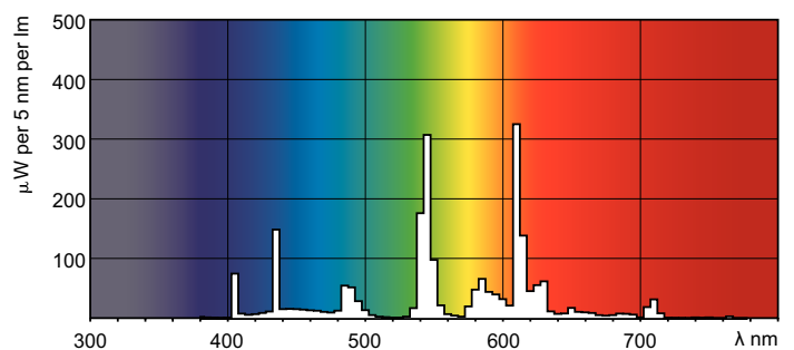
LDPO_PLQ2P_835-Spectral power distribution Colour
