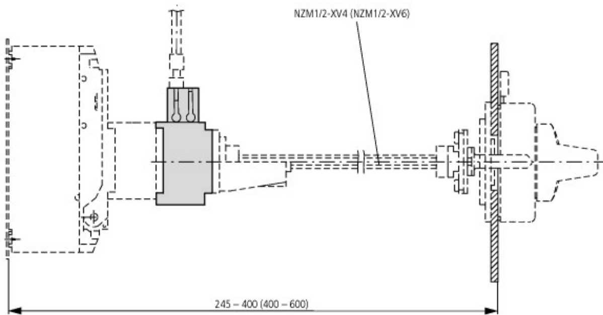
NZM1-XMV + NZM1-XTVD(V)(R)
