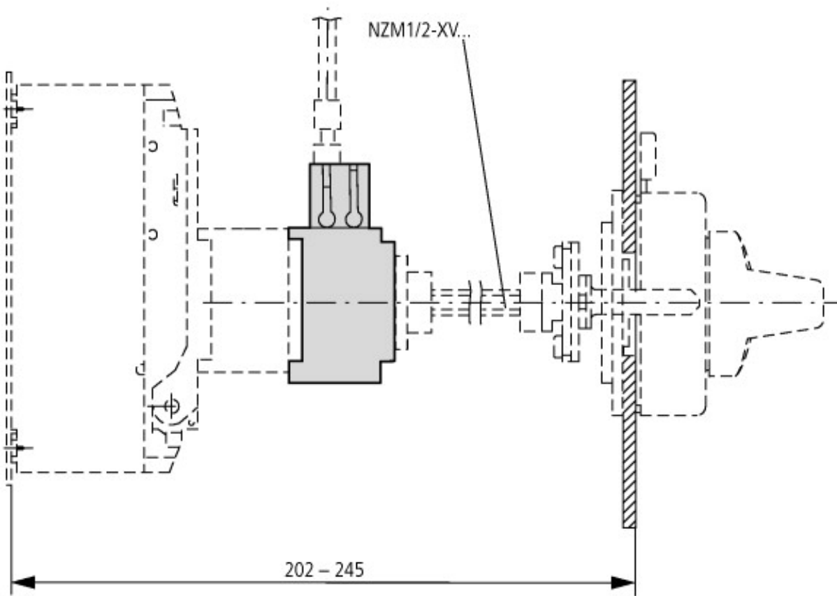
NZM1-XMV + NZM1-XTVD(V)(R)
