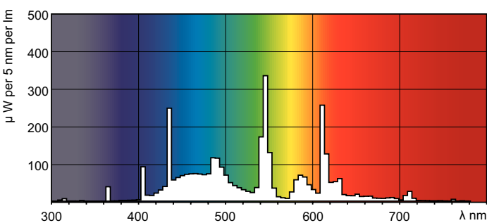
LDPO_TL-D9HLM_965-Spectral power distribution Colour
