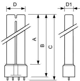
PL-L 18W/827/4P
