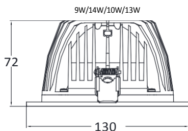
LEDDownlightRc-HM R120
