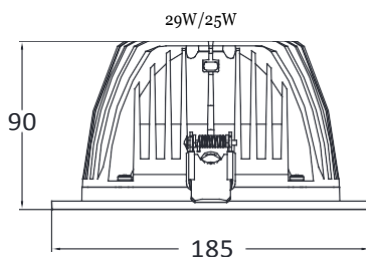
LEDDownlightRc-HM R175
