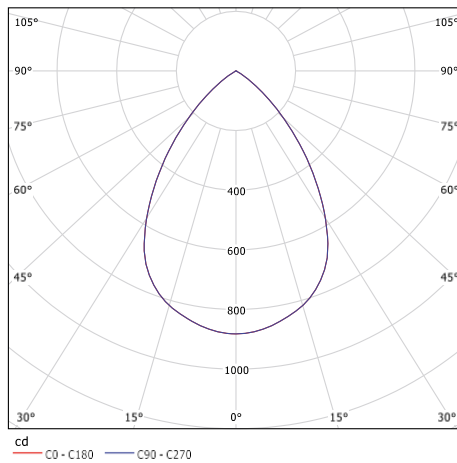
42W-4000K
