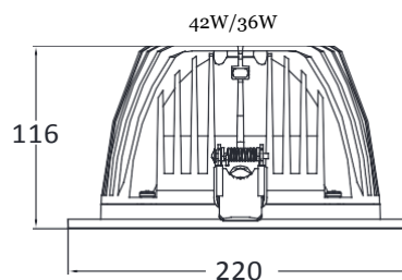
LEDDownlightRc-HM R210
