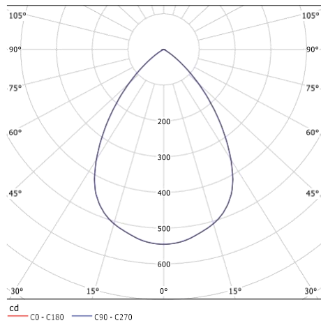
29W-4000K
