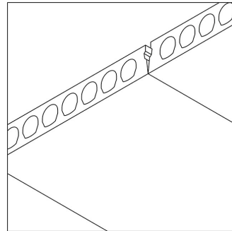
Hollow-core slab
