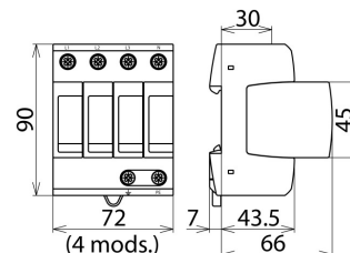
Dimensions DG M TNS CI 275
