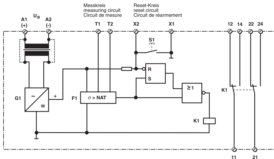
Fig. 1: Wiring diagram
