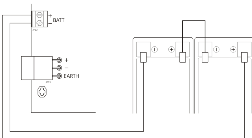
Figure 7 : Raccordement des batteries
